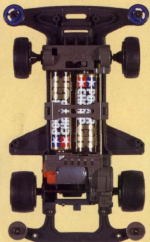
SUPER TZX CHASSIS
